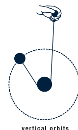
vertical orbits
